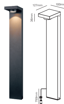
Tide (14.6365.04) 12V | 6W | IP54 | 2700K
