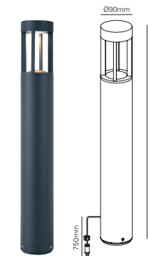
Flow (14.6370.04) 12V | 6W | IP54 | 2700K
