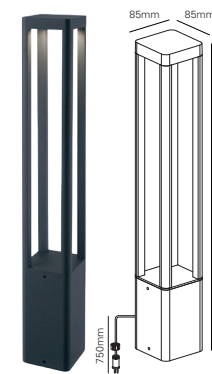
Eclipse floor IV (14.6310.04) 12V | 3W | IP54 | 2700K
