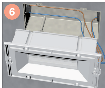
Close the back-door and insert the light body in the back-box. Pay attention to relocate the wiring inside
