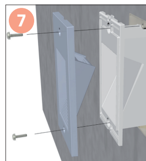
Block the external mask and the light body to the back-box
