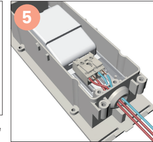
Operate in order to keep the membrane around the cable towards out
