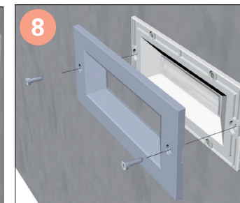
IP65 index is guaranteed only if the back-box is completely in line with the surface of the wall. If it's not so, you can use the additional gasket supplied, in order to compensate the level difference
