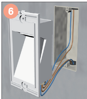
Close the back-door and insert the light body in the back-box. Pay attention to relocate the wiring inside
