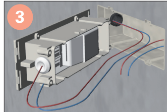
Insert the power conductors through the membrane cable entry and connect to the pushwire terminal block. In case of through wiring installation use the two cable entry / each terminal
