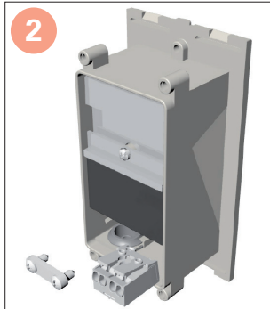
Insert the power conductors through the membrane cable entry and connect to the pushwire terminal block. In case of through wiring installation use the two cable entry / each terminal
