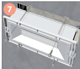
Block the external mask and the light body to the back-box
