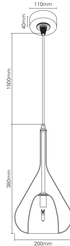
IONIA PENDANT 1-L , glass E Art.nr.: 13.7075.04, Black canopy & brown glass
