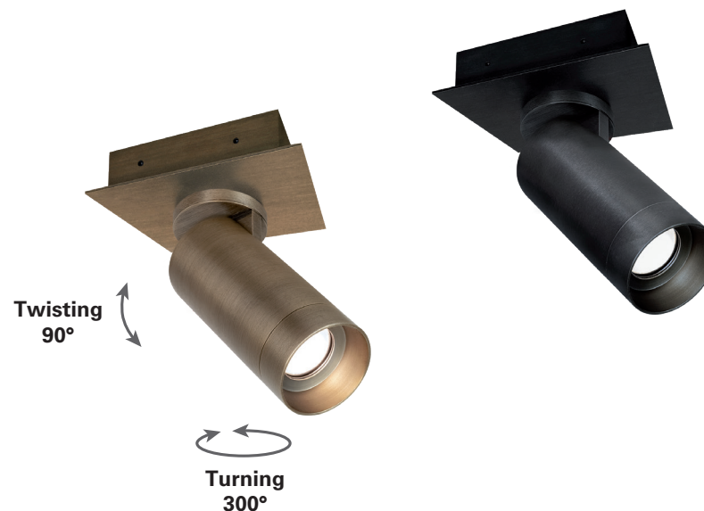
ADJUSTABLE BEAM ANGLE (NARROW TO WIDE)
