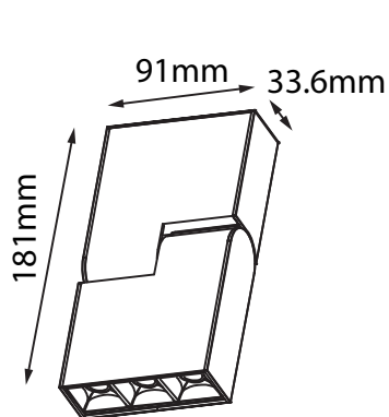
12.5440.04.A MagneTrack Piega 3
