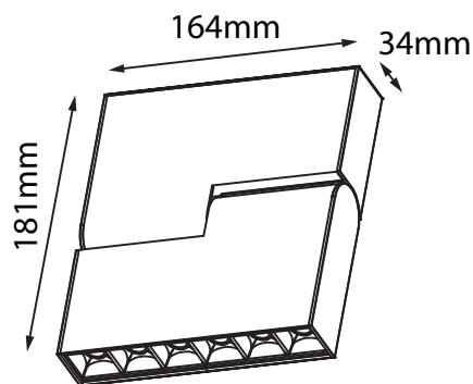
12.5442.04.A MagneTrack Piega 6
