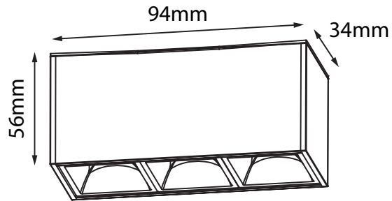
12.5432.04.A MagneTrack Stella 3
