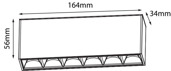
12.5434.04.A MagneTrack Stella 6
