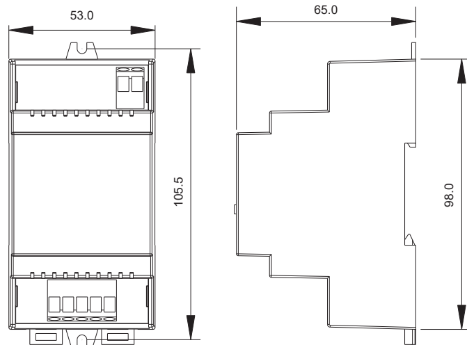
DALI Power supply 250mA DIN RAIL 100.0084.34
